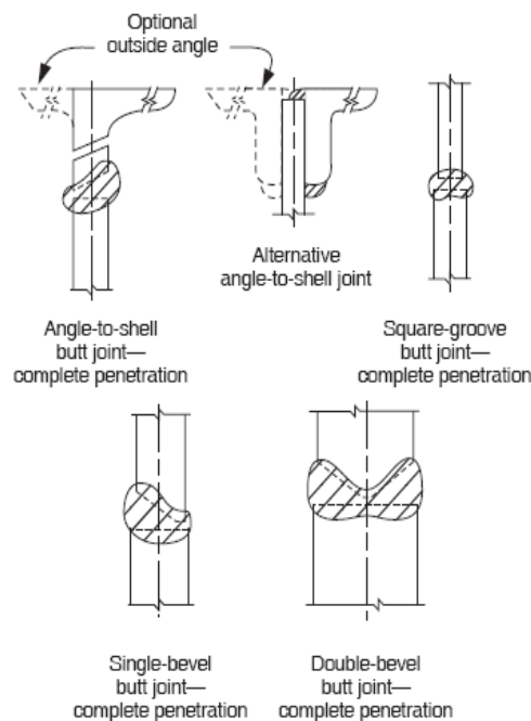
Figure 5-2—Typical Horizontal Shell Joints
