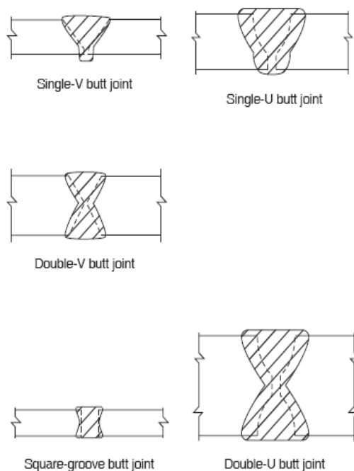
Figure 5-1—Typical Vertical Shell Joints
